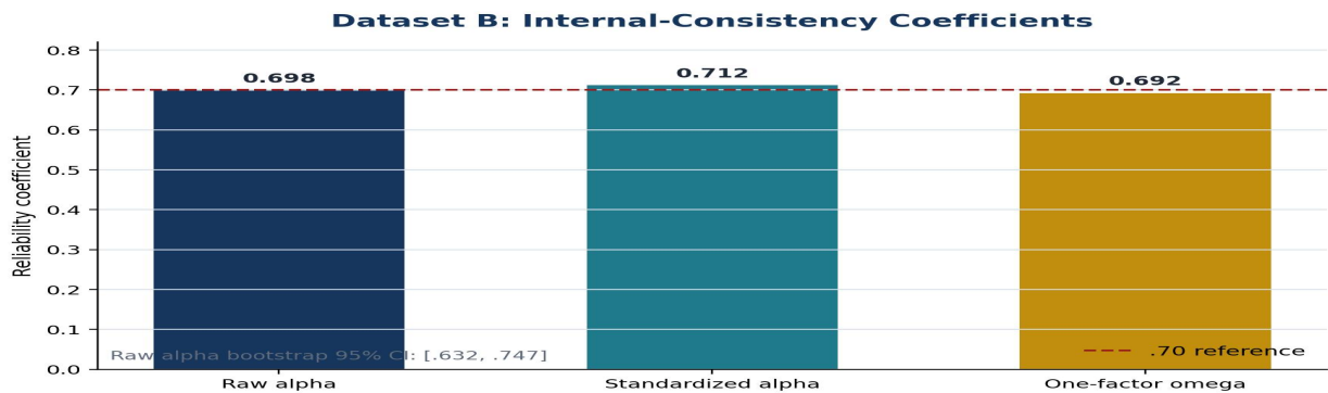
Figure 3: Raw alpha, standardized alpha, and one-factor omega in Dataset B; the dashed line marks .70.
